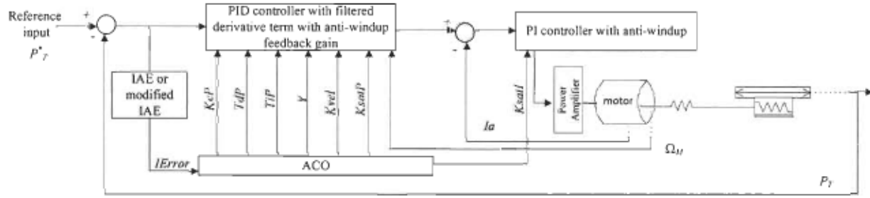
Figure 1- System overview with ACO application for PID parameters tuning
