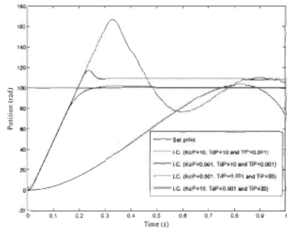
Fig. 9. Step response for the PID controller for the grinder position ( \sigma=1 ) using different initial conditions for NM algorithm.
