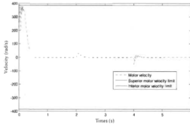
Fig. 15: Motor velocity with saturation compensation; K_r = 0.075 .
