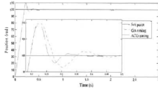
Fig. 12- Input and disturbance steps response and enlargement of input step response for weighted PID controller ( \sigma = 2 , K_t = 0.75 )- ACO vs GA tuning
