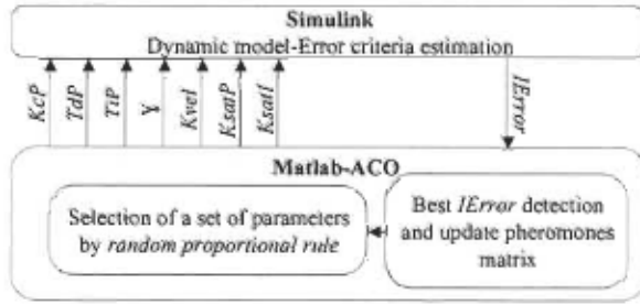
Figure 4- Simulation environment structure of ACO iteration
