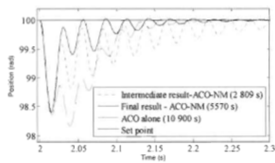
Fig. 13- Enlargement of disturbance response.
