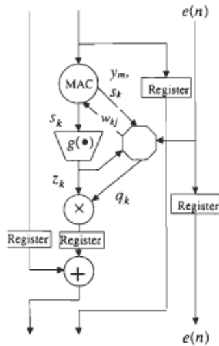
Figure 4: The processing element PE_k .
