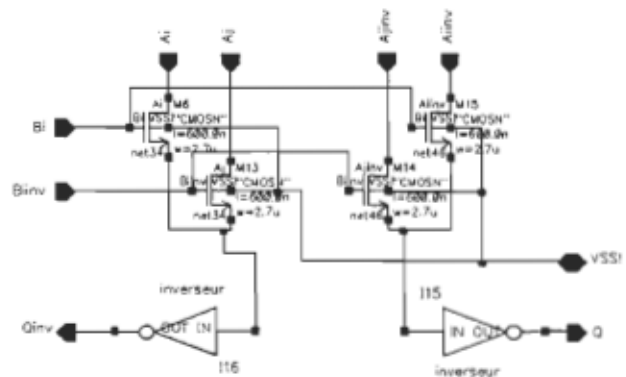
Figure 4: Structure of the NPCPL
