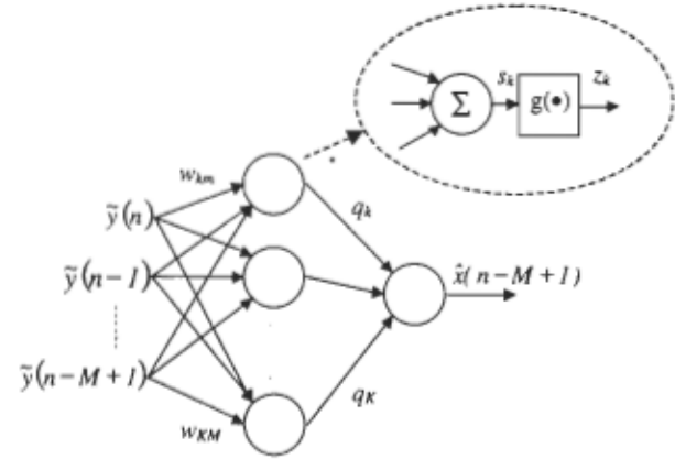
Figure 2: The structure of the neural network (PL-MNN).
