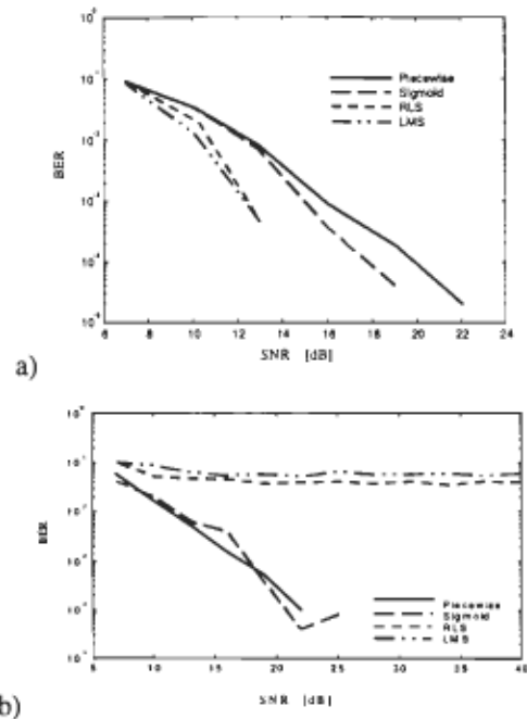
Figure 5 : Robustness of noise for the linear channel (a) and the nonlinear channel (b) with an on-line training of 5 000 iterations.
