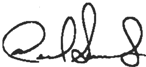
Figure 4.5: Signature S.
