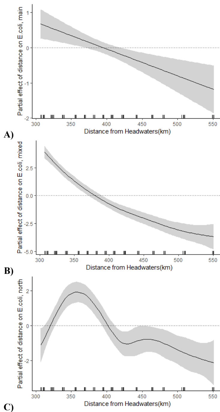
Figure 3.3 Generalized Additive Model (GAM) describing the partial effect of distance from headwaters (km) on E. coli concentration (CFU per 100 mL) across different water masses in the Lower St. Lawrence River while accounting for the random effect of year. A) Main water mass. B) Mixed water mass. C) North water mass. The shaded area indicates the 95% confidence interval, dashed line indicates the null effect, and the rug plot (tick line on the x axis) are the observations of the predictor variables.
