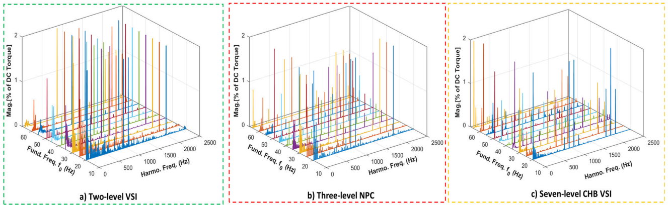
FIGURE 15. Simulation results with synchronized PWM; f_c = 1\text{ kHz} ; f_0 = 45\text{ Hz} .
