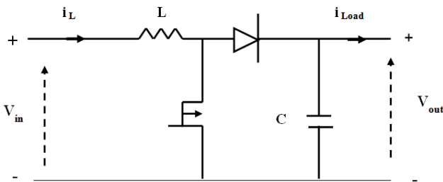
Figure 3. The boost converter's electrical mode [17]
