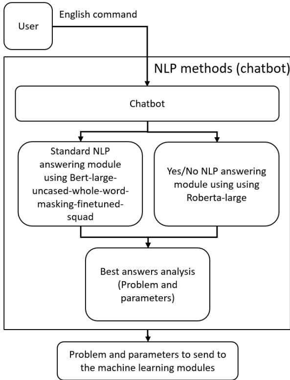
Fig. 2: Architecture of the NLP interface in the AI 2 framework.
