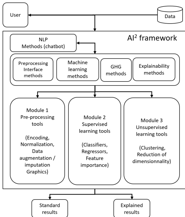
Fig. 1: Architecture of the AI 2 framework.
