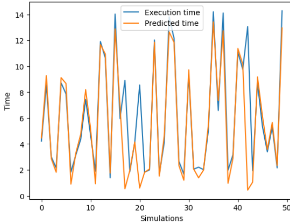
Fig. 9: Validation of the predicted and real execution time
