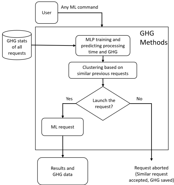
Fig. 6: GHG module architecture
