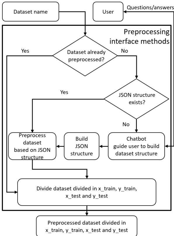
Fig. 3: Preprocessing architecture
