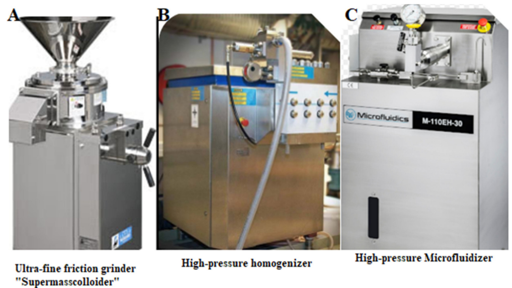
Figure 4. The three most common mechanical devices for the production of CNFs and LCNFs. (A) Ultrafine grinder, (B) high pressure homogenizer (HPH), and (C) high pressure microfluidizer (HPM).
