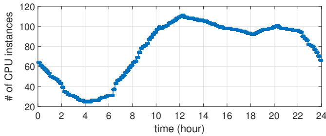
Fig. 9: Total number of processing instances required by the Slice Orchestrator System to met the delay budget (2 ms).
