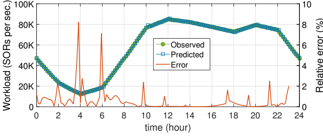
Fig. 5: The temporal distribution of the workload profile (expressed in slices orchestration requests -SORs- per second) and the prediction error of the workload predictor.
