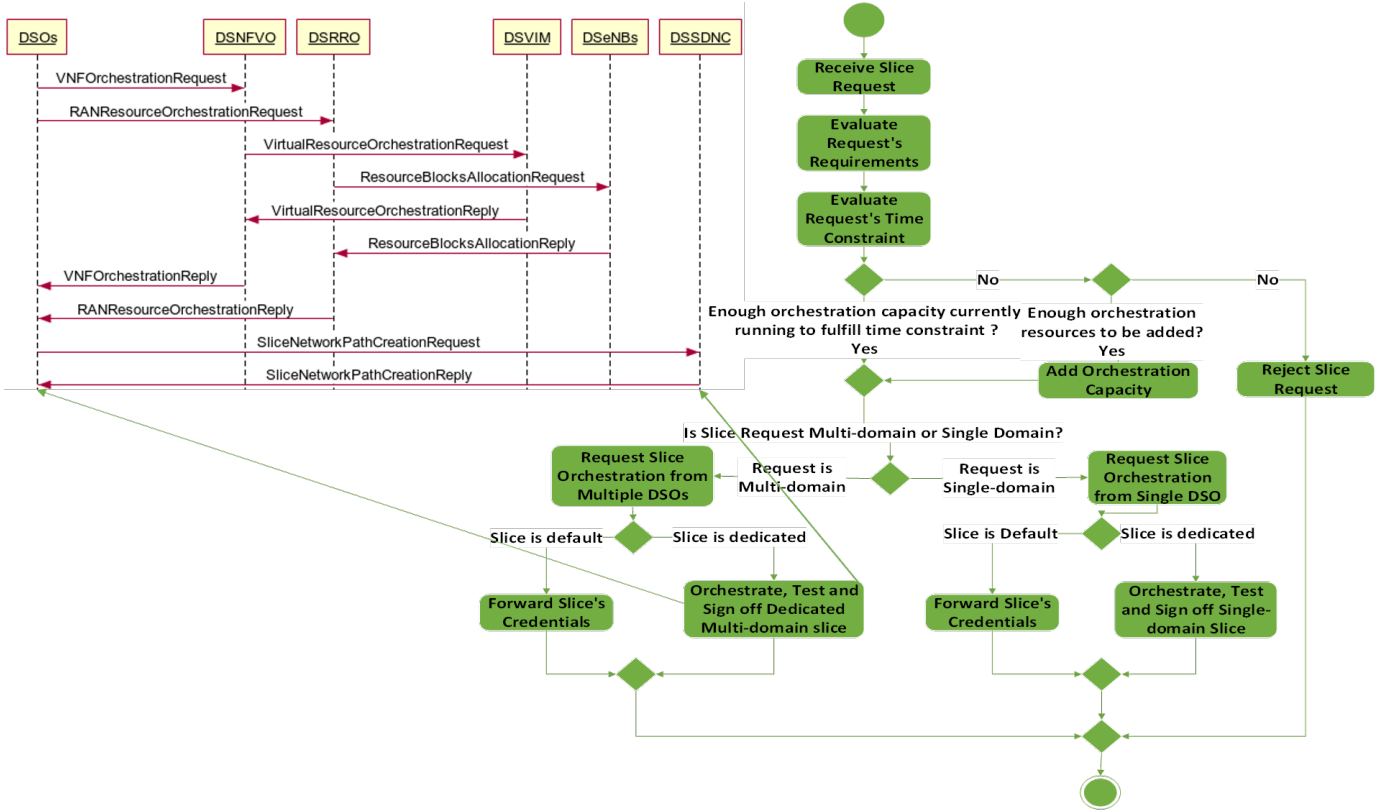
Fig. 2: Activity diagram of the Global Orchestrator.
