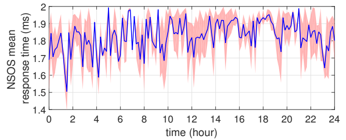
Fig. 11: Slices Orchestration System response time.
