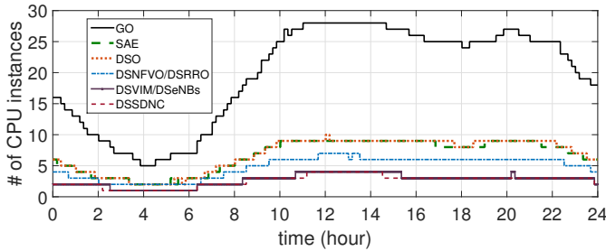
Fig. 10: Number of processing instances allocated to each entity to met the delay budget (2 ms).
