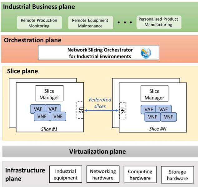
Fig. 2. Framework architecture for the orchestration of industrial network slices.
