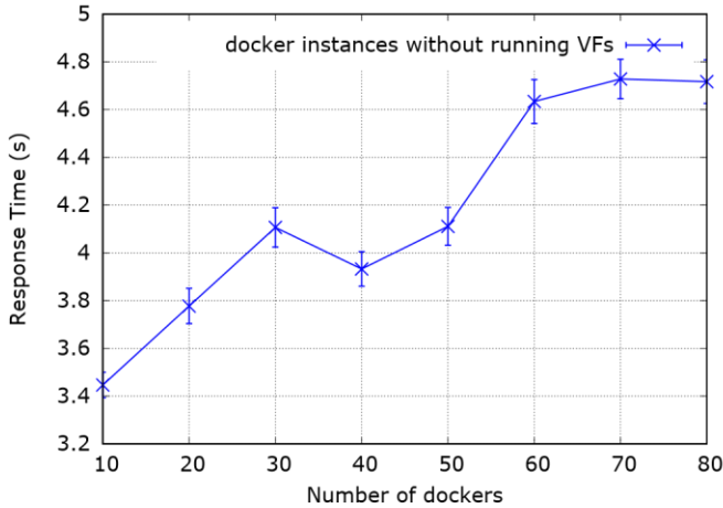
(a) Case of newly-created empty docker instances.
