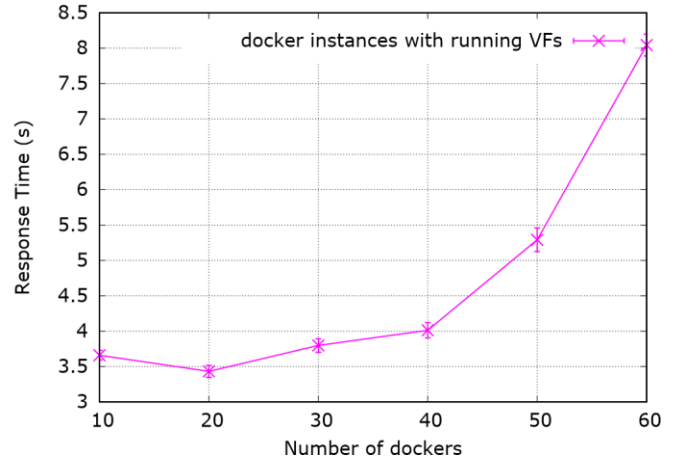
(b) Case of docker instances newly-created with actually running VNFs.
