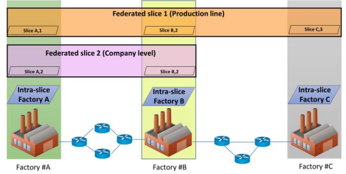
Fig. 1. Federations of industrial network slices over heterogeneous factory infrastructures.
