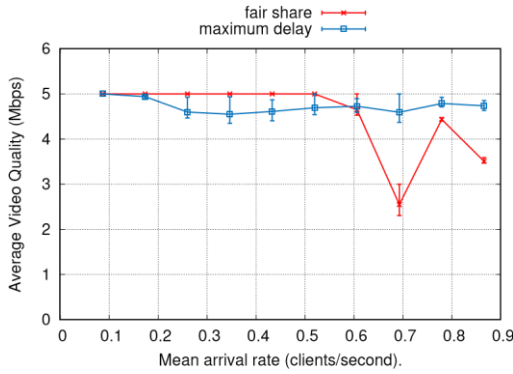
Fig. 5: Overall average video quality for accepted clients.
