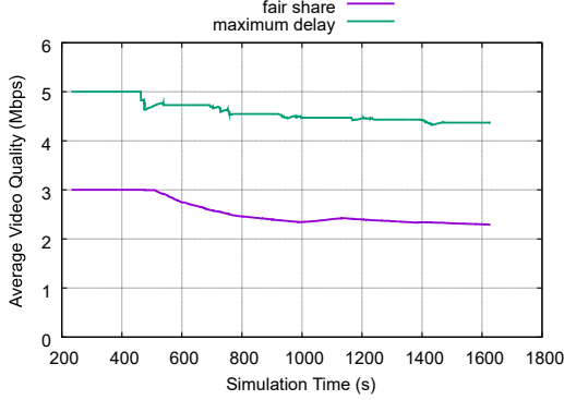
Fig. 4: Average quality for 160 incoming clients' arrival rate.
