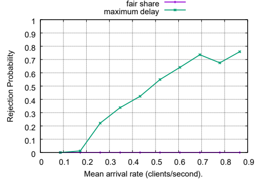
Fig. 6: Rejection Probability.
