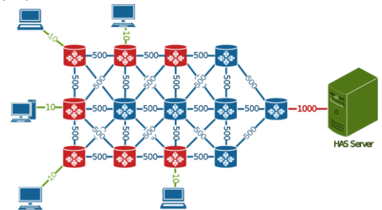
Fig. 3: Simulation Setup.
