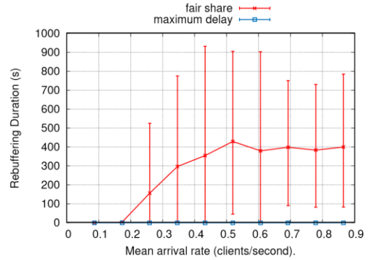
Fig. 7: Cumulative rebuffering duration.
