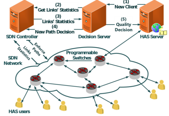
Fig. 2: System Architecture.
