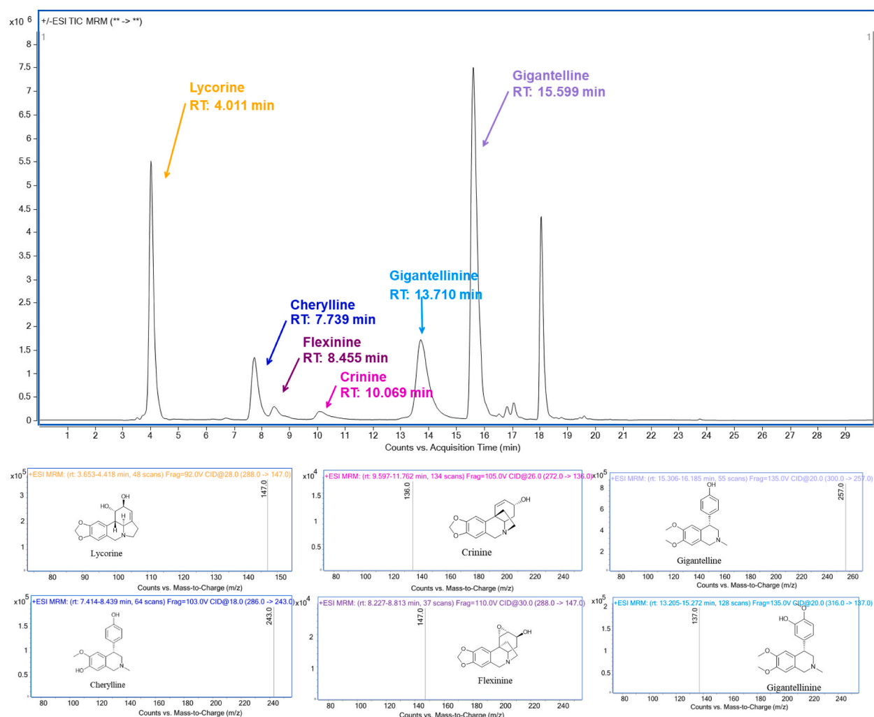
Fig. 2. Total Ion Chromatogram (TIC) of Crinum jagus extract analyzed by HPLC-MS/MS and MS of selected alkaloids. The TIC shows the relative abundance of ions detected over time, with peaks corresponding to individual compounds. The major alkaloids identified in the extract are labeled: cherylline, flexinine, crinine, lycorine, gigantellinine, and gigantelline. The retention time of each compound is indicated on the x-axis. MS is provided indicating its mass ion peak and structure.
