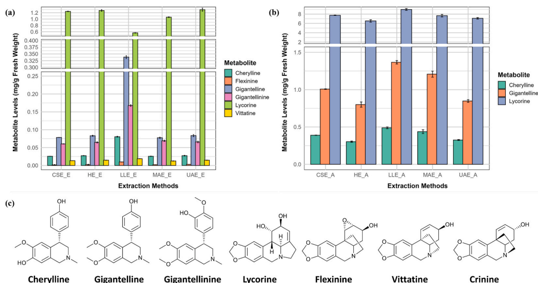
Fig. 1. Alkaloid content and chemical structures of Crinum jagus extracts prepared using various extraction methods. (a) and (b) show the alkaloid content of extracts obtained using continuous shaking extraction (CSE), hot extraction (HE), microwave-assisted extraction (MAE), ultrasound-assisted extraction (UAE), and liquid-liquid extraction (LLE). Methanol extraction is represented by E and subsequent acid-base extraction are denoted by A. (c) shows the chemical structures of the alkaloids cherylline, gigantelline, gigantellinine, lycorine, flexinine, vittatine, and crinine. Data represent the mean \pm standard deviation ( n = 3 ). Different letters above the bars indicate significant differences ( p < 0.05 ) according to Turkey's test. FW: fresh weight.
