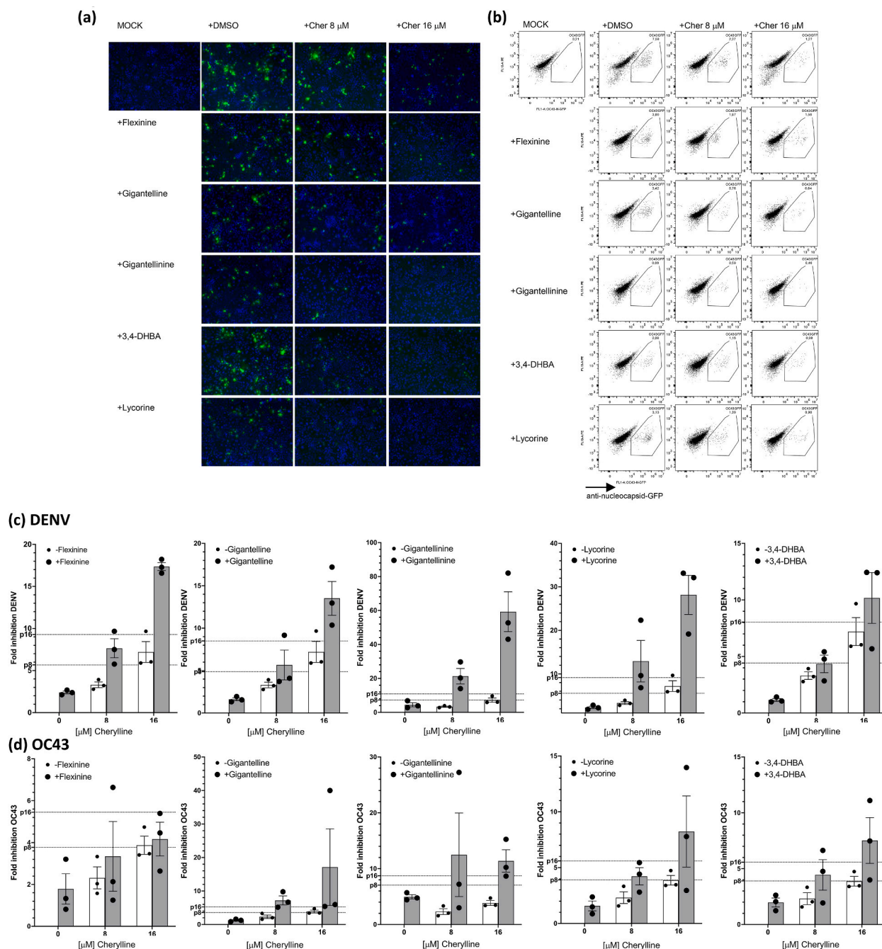
Fig. 7. Antiviral activity of Crinum jagus specialized metabolites. (a): Anti-flavivirus activity of single and combination of AAs extracted. Inverted microscope merged images taken at 5X of Huh7 cells stained with Hoechst333642 (nucleus, blue) and infected with DENV GFP (green). (b) Anti-coronavirus activity of single or combined AAs and 3,4-DHBA. Flow cytometry dot plots of HCT8 cells infected with HCoV-OC43 treated with a combination of DMSO (0.1 %) or cherylline (8 or 16 \mu M), and flexinine (150 \mu M), gigantelline (150 \mu M), gigantellinine (150 \mu M), 3,4-DHBA (25 \mu M), or lycorine (0.25 \mu M). Cells were trypsinized, fixed, permeabilized, and stained with an anti-nucleocapsid antibody (green) and a secondary antibody, and with hoechst333642 to gate on intact cells. Shown are representative pictures and dot plots on three biological replicates. (c) C. jagus AA synergistic effects on DENV inhibition. The % of infected cells was assessed by flow cytometry 72 h post-infection. (d) Combination of metabolites inhibitory effect against anti-betacoronavirus (HCoV-OC43). HCT-8 were used as target of OC43 infection, while Huh7 were used for DENV. Shown are means with SEM.
