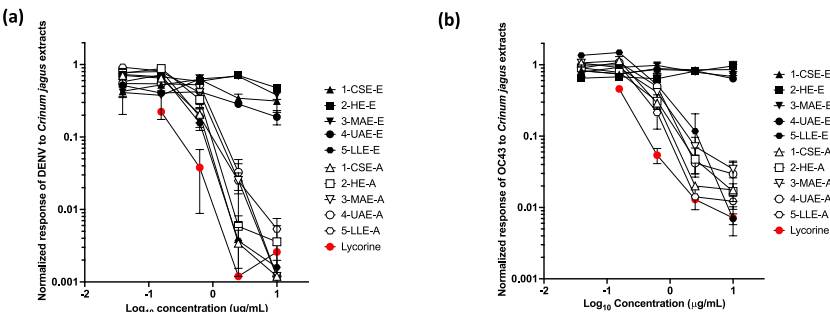
Fig. 5. Antiviral properties of Crinum jagus extracts. (a) Anti-flavivirus (DENV) activity in Huh7 cells. (b) Anti-betacoronavirus (HCoV-OC43) activity in HCT8 cells. Cells were treated with the fractions and infected with the corresponding virus at on MOI of 0.1 (DENV) or 0.01 (OC43). Huh7 cells were trypsinized, fixed and analyzed by flow cytometry 72 h post-infection. HCT8 cells were trypsinized, fixed, permeabilized, and stained with an anti-nucleocapsid antibody (green), secondary antibody and with hoechst33642 96 h post-infection. The % of infected cells was assessed by flow cytometry and normalized to the % of untreated control to yield the relative infection levels. Shown are means of biological triplicates ± SD.
