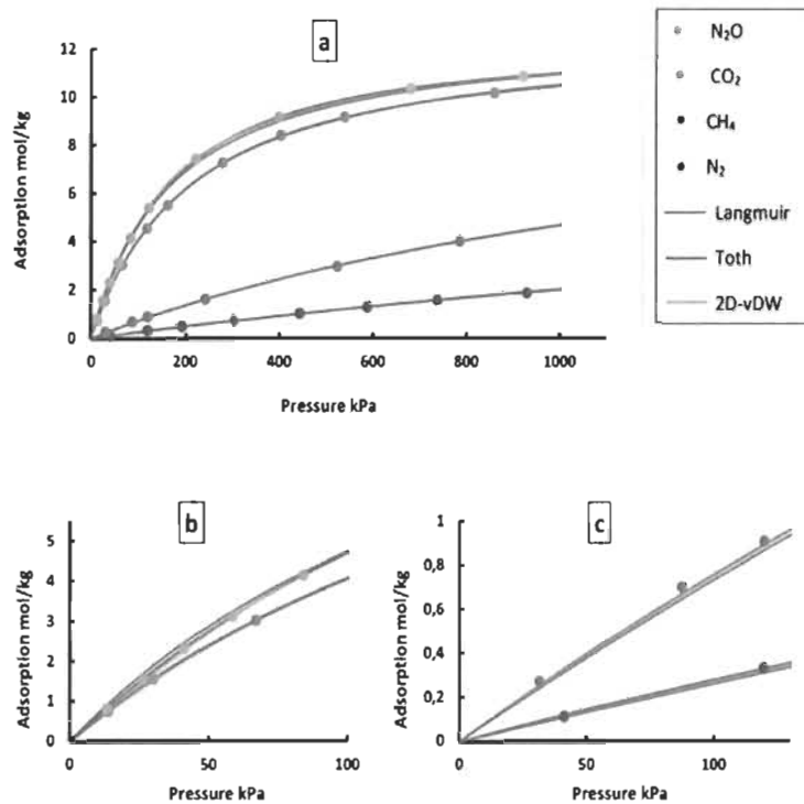
Figure 1 Single-component adsorption isotherms of N 2 O, CO 2 , CH 4 and N 2 : a) Full pressure range (0-1000 kPa); b) 0-100 kPa for N 2 O and CO 2 ; c) 0-100 kPa for CH 4 and N 2 . Points are experimental data while solid lines are models.
