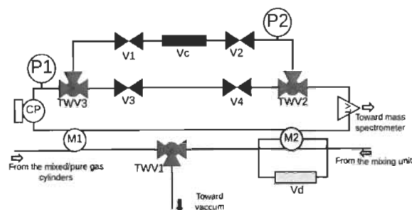
Fig. 1 Schematic representation of the adsorption section. P1, P2: Digital pressure transducers (HEISE DXD 0-500 PSIA). Vd: dosing volume, TWV1: Swagelok 3-way valve 42GX series, Vc: adsorption chamber volume, TWV2, TWV3: Swagelok 3-way valve 41GX series, V1, V2, V3, V4: Swagelok ball valves 43GS8-31C, LV: Leak valve SS22RS2, CP: Magnetic circulation pump (MICRO-PUMP GAH-SERIES)
