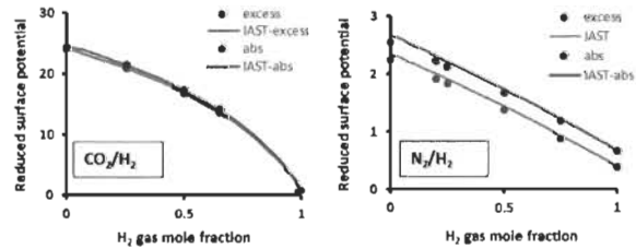
Fig. 12 Comparison of absolute and excess surface potential
