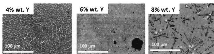
Figure 1. Backscattered micrographs of the as synthesized alloy of Ti-Fe + x wt.% Y (x = 4, 6, and 8).
