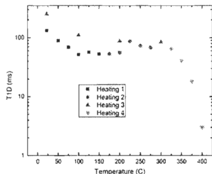
Fig. 8. Relaxation time T_{1D} versus temperature for cold rolled MgH_2 .
