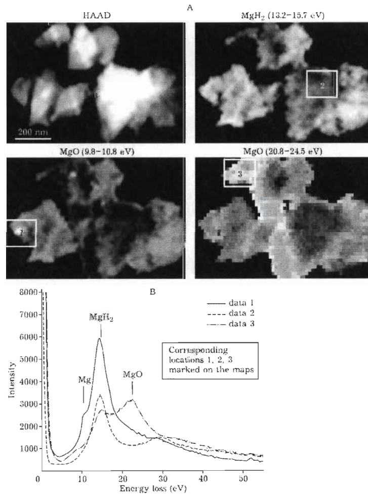
Fig. 7. (A) STEM-HAADF image of MgH_2 cold rolled in argon for 75 times along with energy-filtered maps corresponding to the various phases present. The energy range used for each map is given in the brackets. (B) EEL spectra from three locations, marked on the maps shown in (A).
