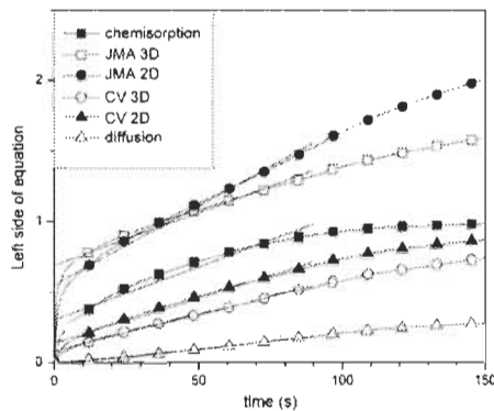
Fig. 3. Rate limiting step curves for the absorption reaction at 623 K, using the equation left sides given in Table 2. The points are data from Fig. 1; the smooth curves connect the points. The straight lines are best linear fits to the data for X between 0.1 and 0.9.
