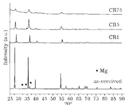
Fig. 2. X-ray diffraction patterns of magnesium hydride as-received and cold rolled in air.
