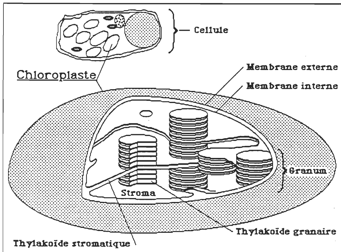
Figure 1. Structure du chloroplaste.
